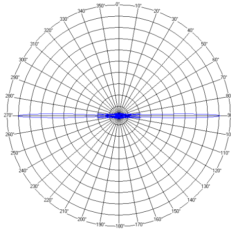
Fig. 4. Set of array factor plots for influence of elements number increase simulation
