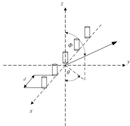
Fig. 1. Schematic diagram of linear antenna array
