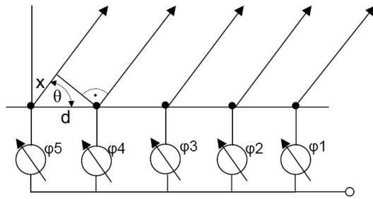
Fig. 2. Schematic diagram of phased linear antenna array beam - steering
