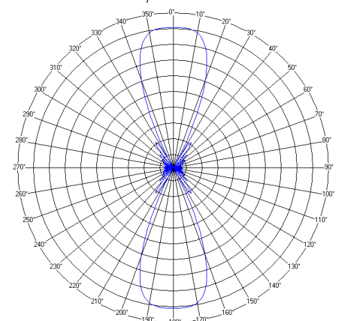
Fig. 5. Set of array factor plots for phase shift change simulation
