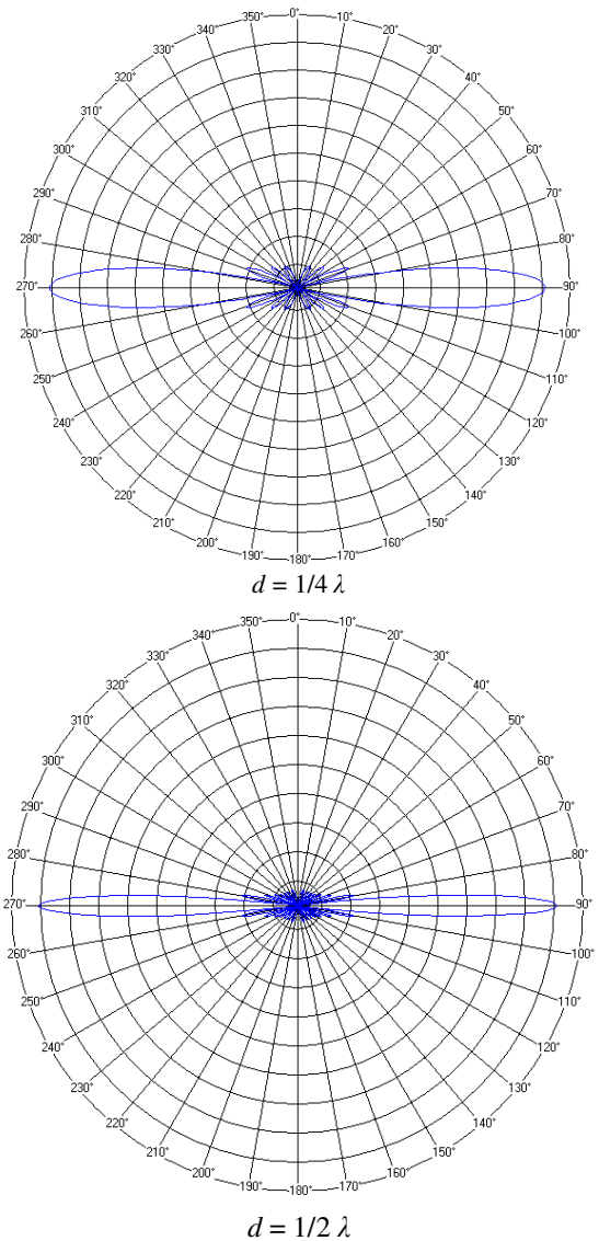
Fig. 3. Set of array factor plots for influence of mutual element's distance simulation
